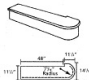
S-8010 Starting Step Reversible 48" Oak
