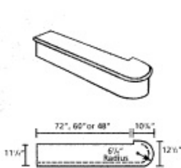
S-8010 Starting Step Reversible Oak - 48", 60" or 72" Paint Grade - 48" Maple - 60"
