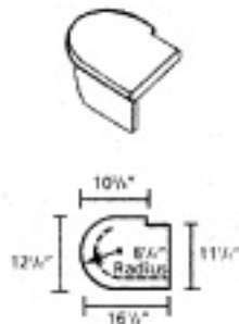
S-8010-2 False Starting Step Reversible Grade or Maple
