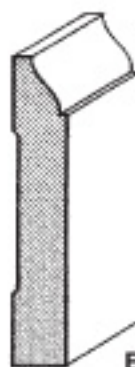
EC623 BASE 9/16" x 3 1/4"
