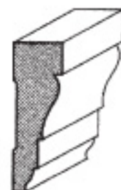
EC366 CASING 1 1/16" x 2 1/4"
